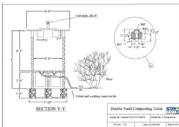
Fig 7: Twin vault UD latrine drawing, Sri Lanka (courtesy ACF)
