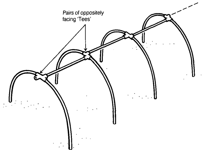
Figure 3. Use of 'Tee' pieces to make greenhouse ridges from PVC pipes
